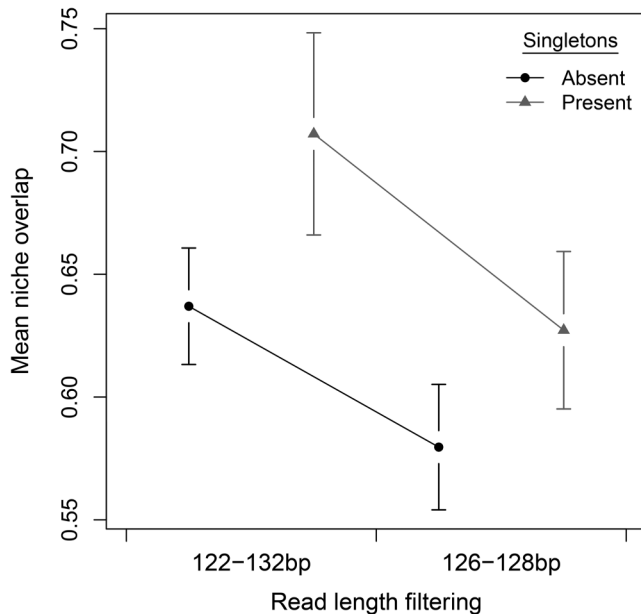
Fig. 6. Significant interaction between the presence or absence of singletons and read length filtering on mean niche overlap; bars are 95% confidence intervals.
