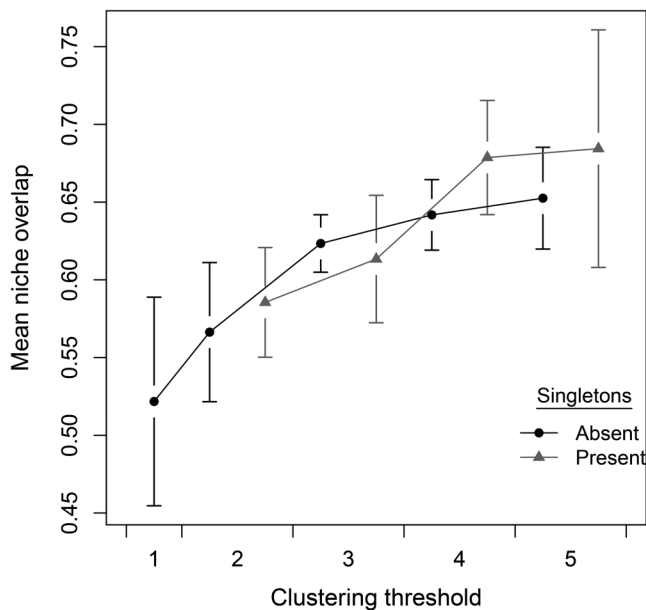
Fig. 4. Significant interaction between clustering divergence threshold (1%–5%) and the presence or absence of singletons on mean niche overlap; bars are 95% confidence intervals. Note: singletons at clustering threshold = 1 generated files too large for analysis and are thus excluded.
