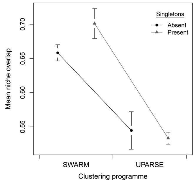
Fig. 3. Interaction between clustering programme (SWARM and UPARSE) and the presence or absence of singletons in the dataset on mean niche overlap; bars are 95% confidence intervals.
