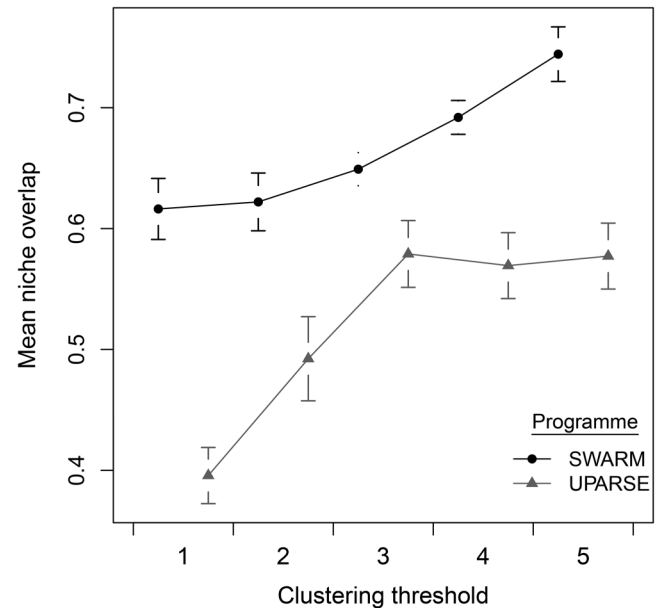
Fig. 5. Significant interaction between clustering divergence threshold (1%–5%) and clustering programme (SWARM or UPARSE) on mean niche overlap; bars are 95% confidence intervals.
