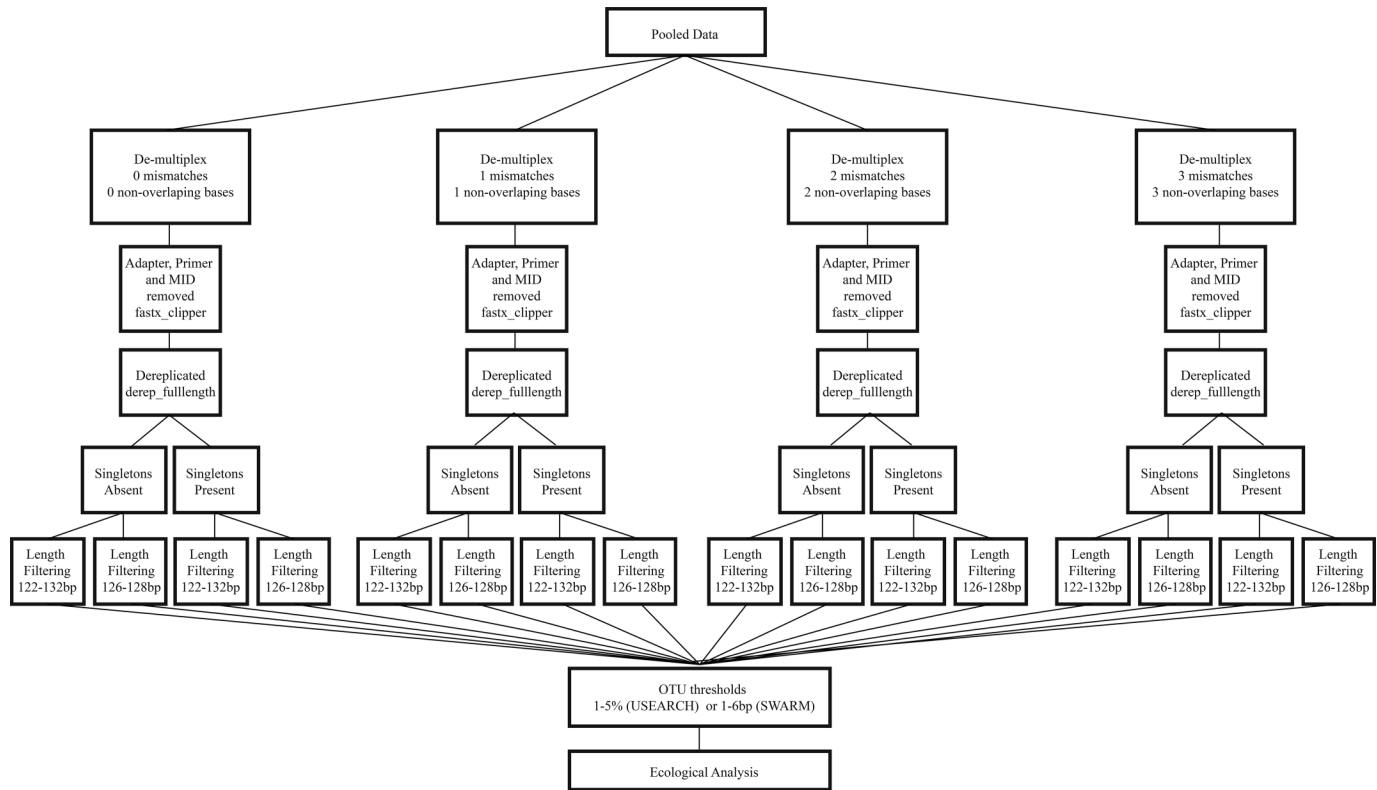
Fig. 1. A diagram demonstrating the variables and analytical steps used in the study design.
